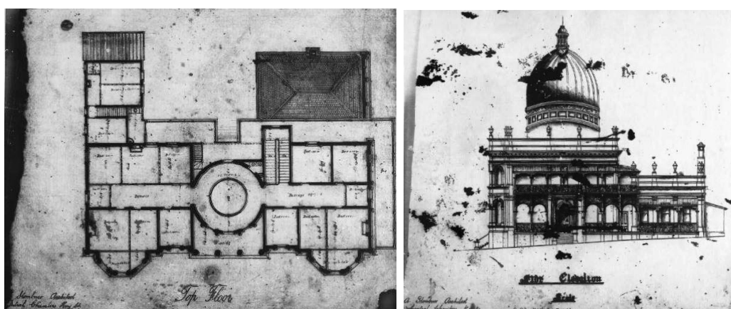
These drawings produced by Stombuco at 'Central Chambers Hay Street' [Perth] are his design for the Weld Club competition of 1891. Reproduced in Carolyn Cox's thesis, Cox notes that the drawings "appear to be of a hotel situated on a corner with entries from both streets", but with the benefit of new research, we now see the drawings provide valuable comparison with the Talbot Hobbs designed Weld Club that was built in Perth. (Cox, C., 'Andrea Stombuco', 1977, p.236, illustrations 8.02-8.03)
